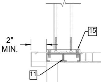
FIXATION ALUMINIUM
